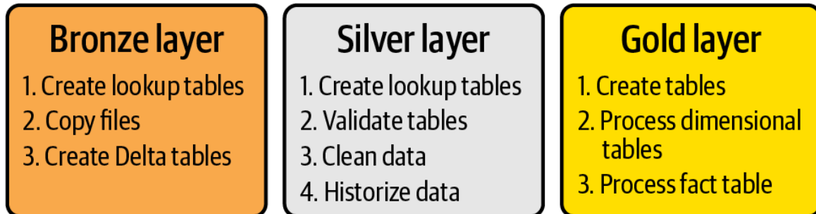
Figure 7-1. The tutorial's overall objectives
