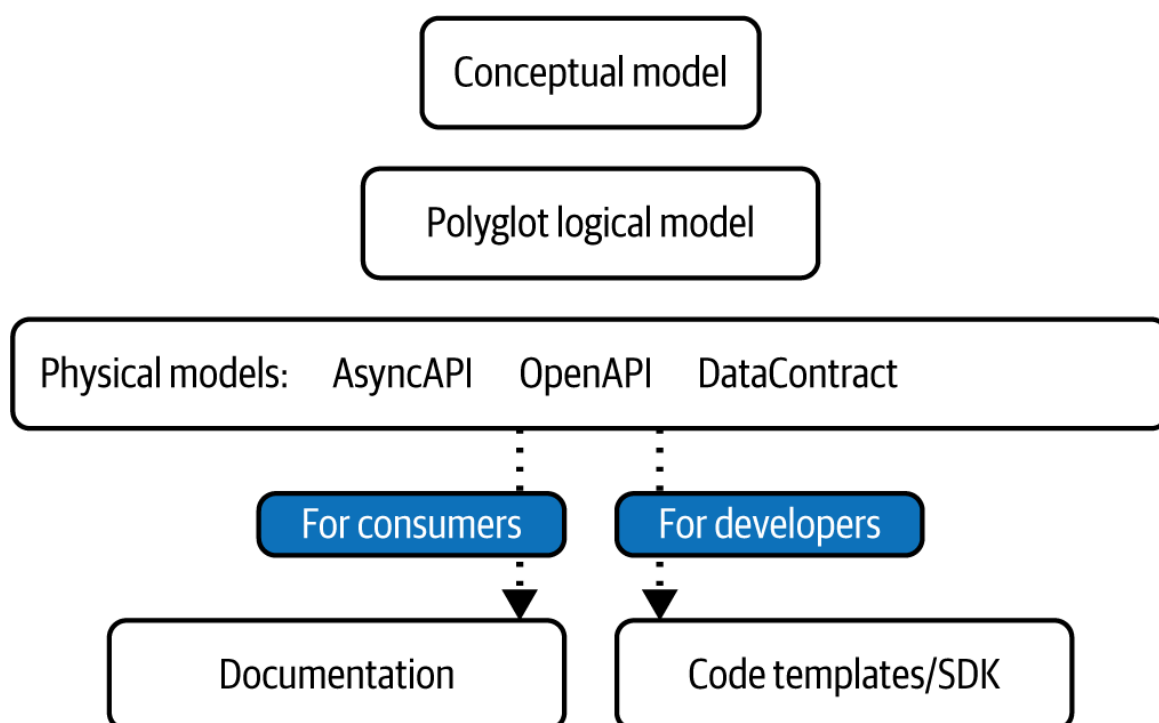
Figure 9-3. Governance is implemented as code by automating the creation of all new interfaces
