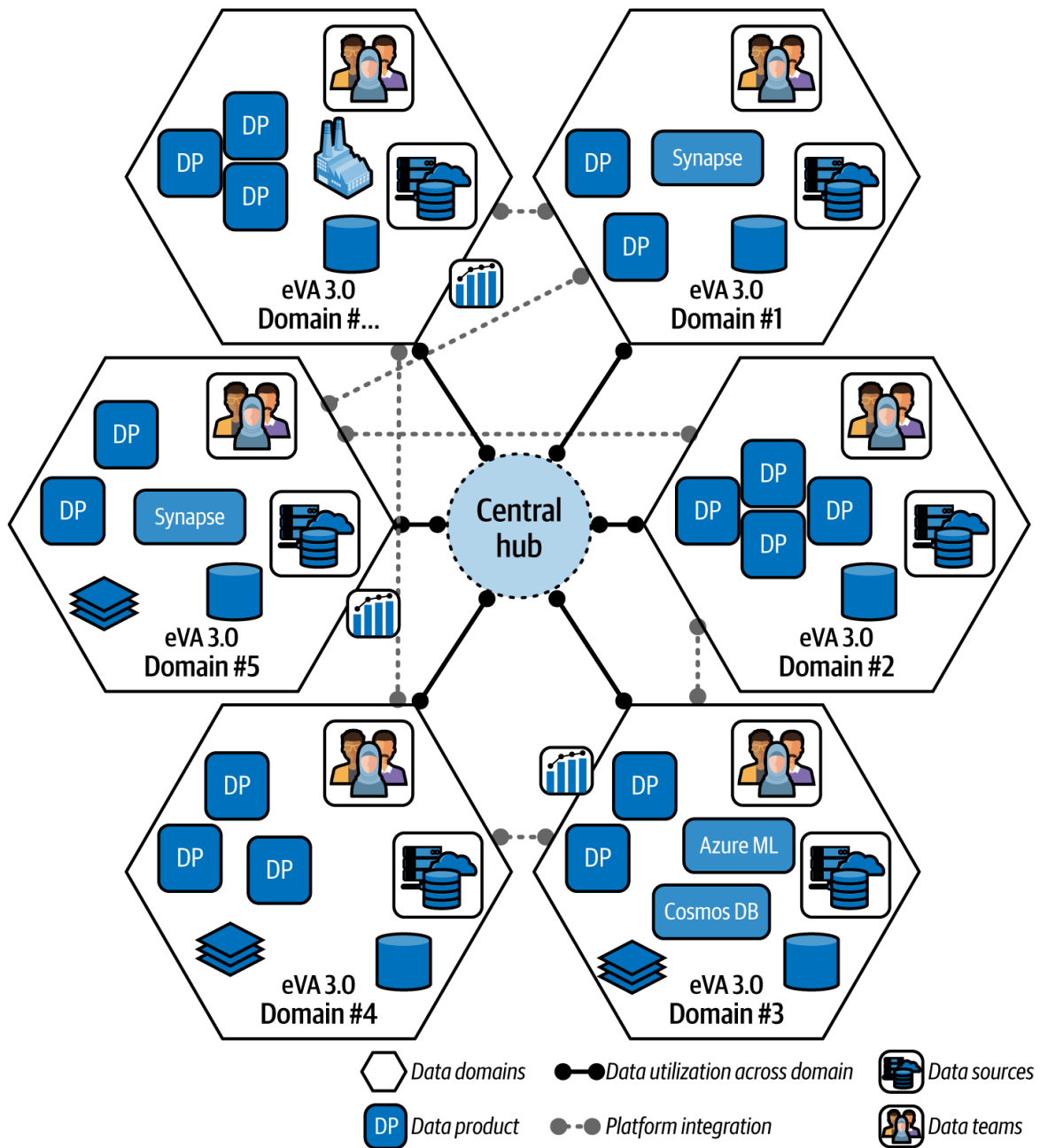
Figure 10-1. High-level overview of the eVa platform
