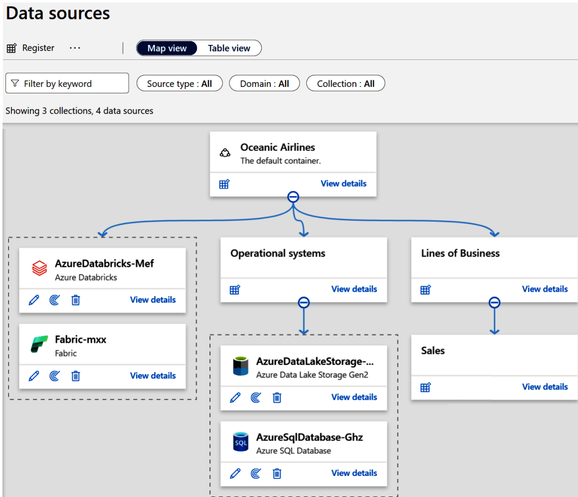
Figure 7-11. Microsoft Purview's Data Sources overview page
