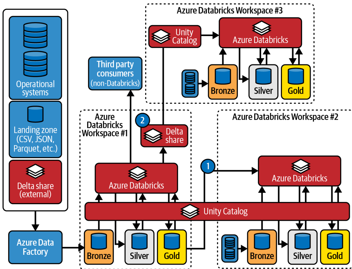
Figure 11-2. A Medallion mesh using Azure Databricks
