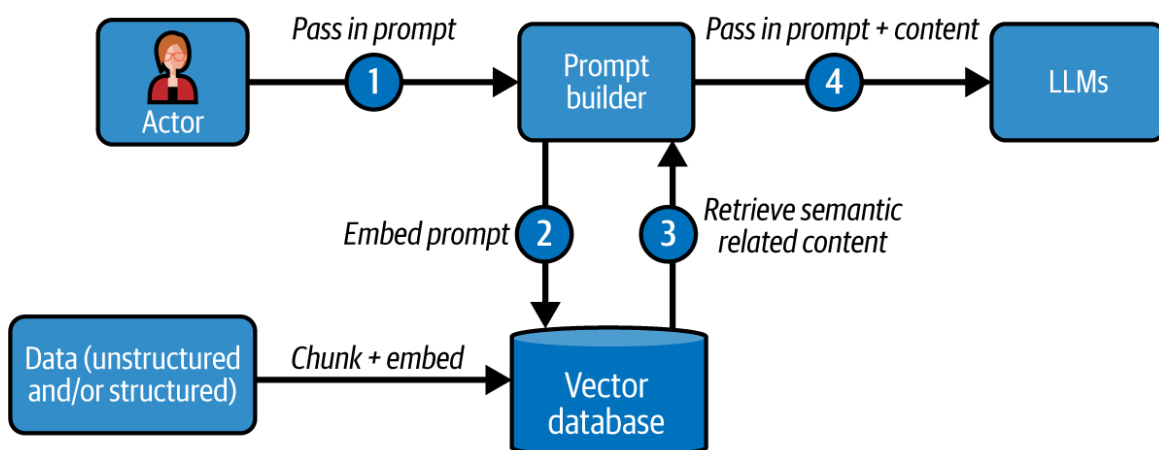
Figure 13-1. The RAG pattern
