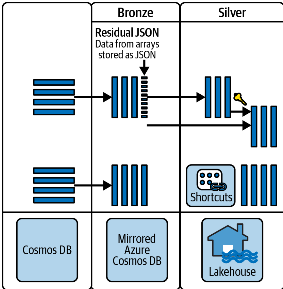
Figure 8-3. High-level overview of AP Pension's deserialization process from a Cosmos DB mirror in Fabric
