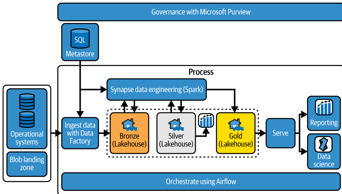
Figure 4-1. High-level architecture design showing proposed architecture
