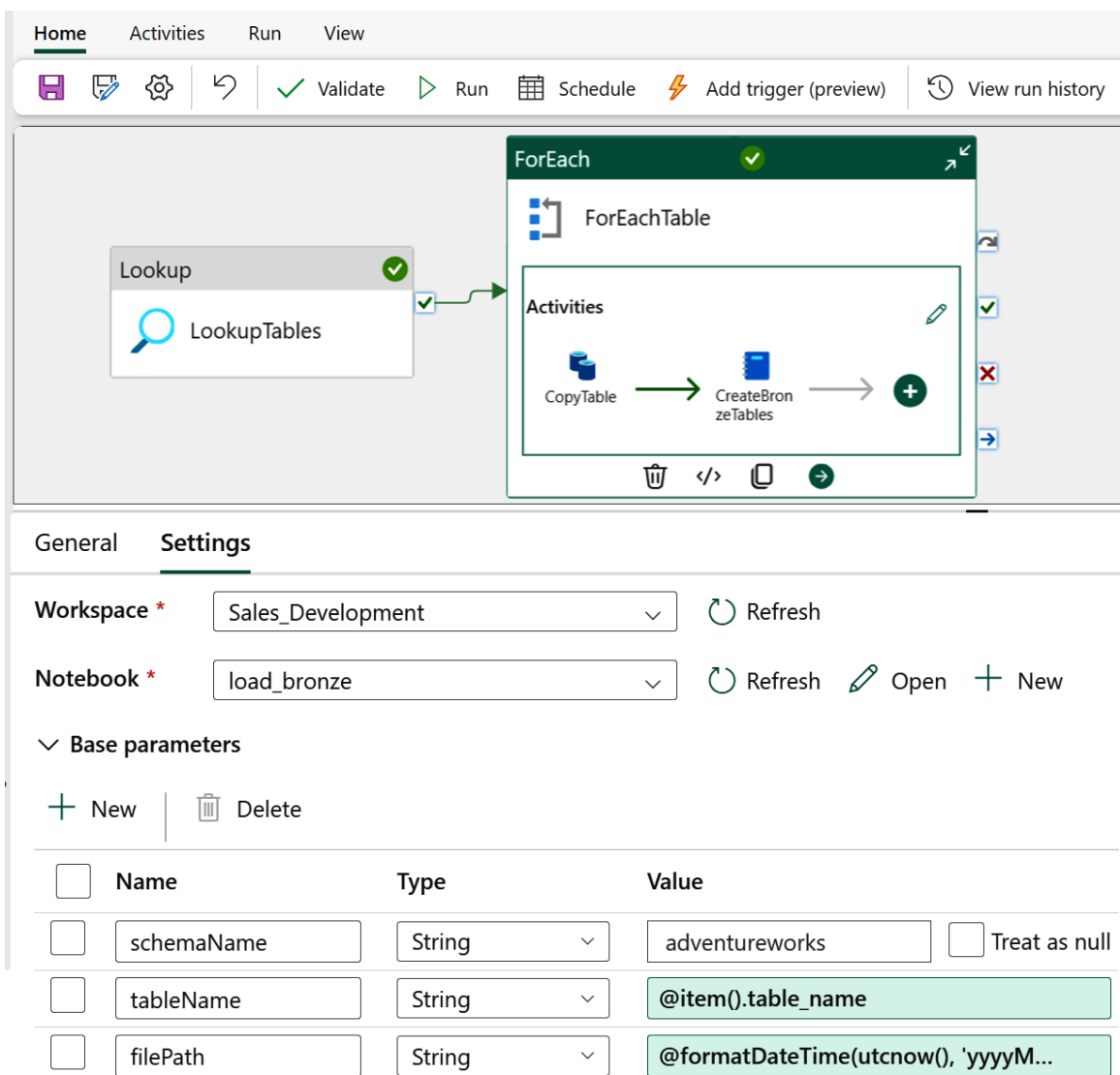
Figure 5-8. Configuration details of the Notebook activity
